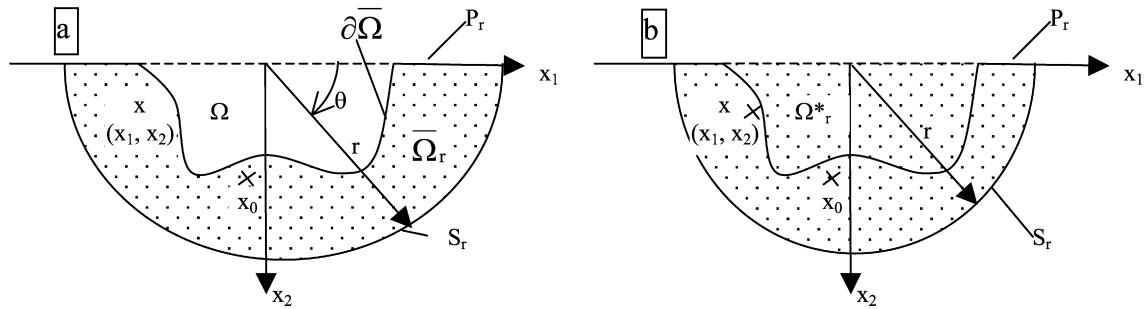
Fig. 1. (a) Integration domain \bar{\Omega}_R (in grey); (b) auxiliary integration domain \Omega_r^* .
