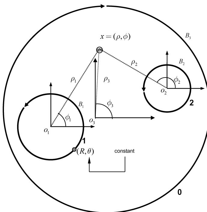
Fig. 2. Adaptive observer system.
