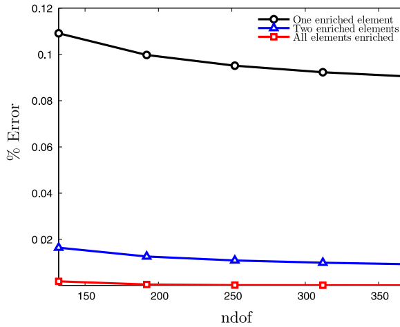
Fig. 7. Effect of the number of enriched elements (Case 1).
