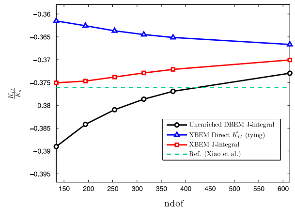
Fig. 15. K_{II} for inclined crack results compared to Xiao et al. [7].
