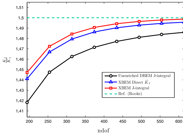
Fig. 12. A comparison of normalised results for bending plate.
