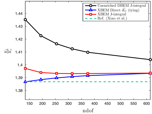
Fig. 14. K_I for inclined crack results compared to Xiao et al. [7].
