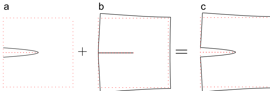
Fig. 4. Displacement components for case 1.
