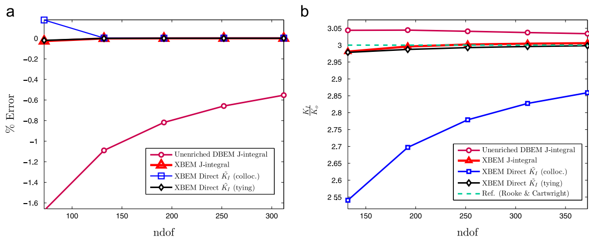
Fig. 6. Results of K_I for Mode I using various methods. (a) Percentage error of K_I for Case 1. (b) Comparison of K_I for Case 2.
