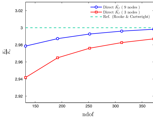
Fig. 8. Effect of order of displacement extrapolation (Case 2).
