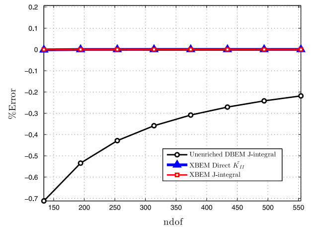
Fig. 10. Results for pure Mode II.
