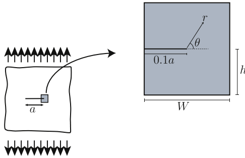
Fig. 2. Infinite flat plate (case 1).
