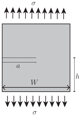
Fig. 3. Square flat plate under axial tension (case 2).
