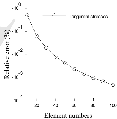
Figure 5: Convergence curve of the computed \sigma_\theta at the point (1\text{E-}9, 0)
