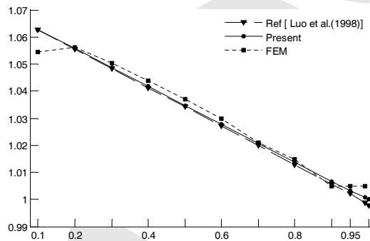
Figure 11: adial stress prediction at the boundary node A.
