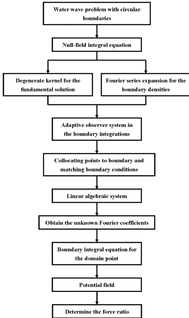
Fig. 5. Flowchart of the present method.
