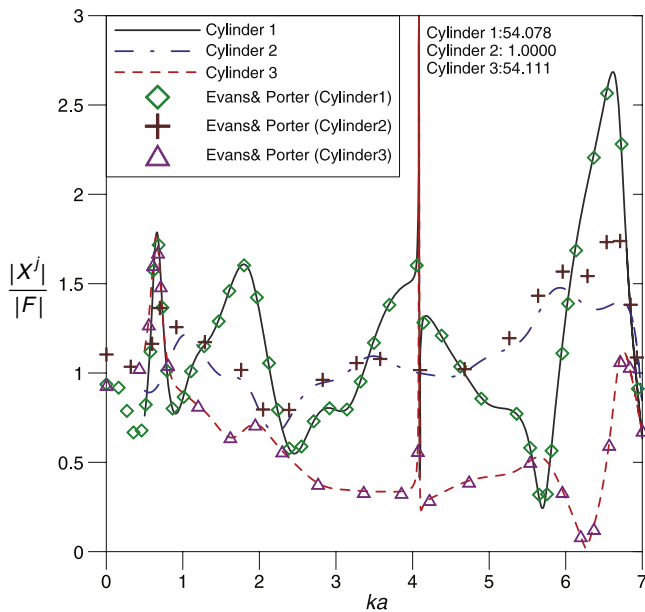
Fig. 10. The force ratio in the direction of wave advance versus wavenumber.
