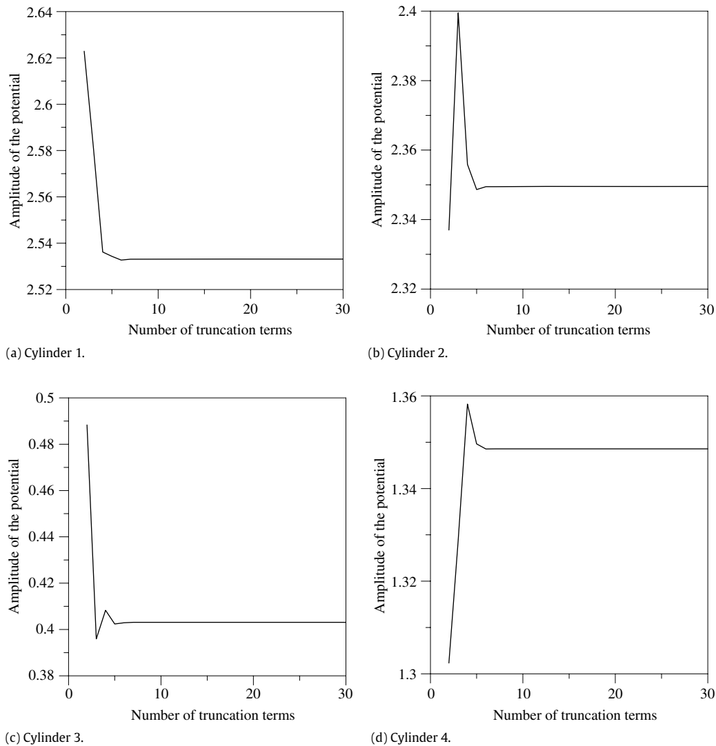
Fig. 9. Amplitude of potentials at north poles versus number of truncation terms on (a) cylinder 1, (b) cylinder 2, (c) cylinder 3 and (d) cylinder 4.
