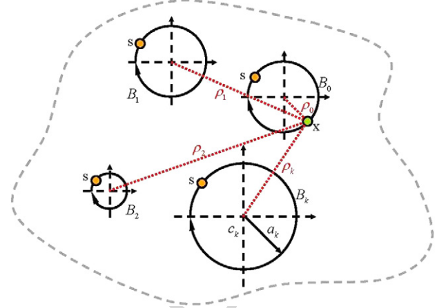
Fig. 2. The adaptive observer system.
